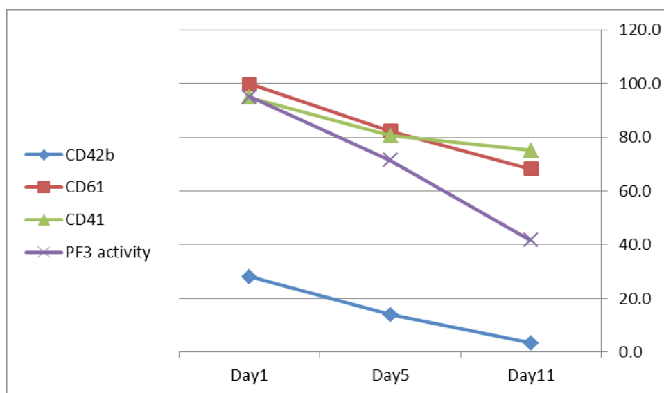
Figure 1: Flow cytometry measurement of CD42b, CD41/CD61 receptors as well as the results of PF3 clotting activity assay during storage of platelet concentrates for eleven days.
