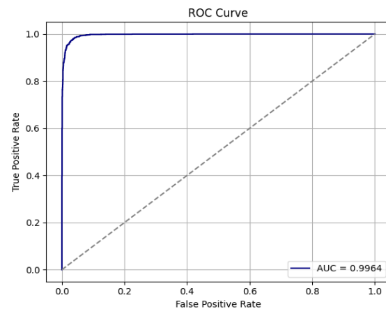
Figure 12. Shows the AUC_Roc Curve: Demonstrating the model's ability to distinguish between classes.
