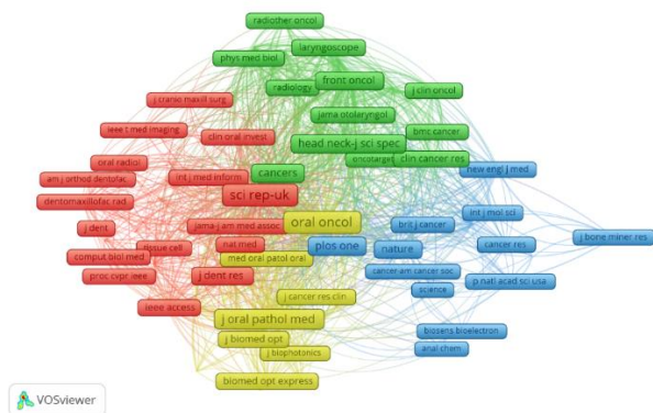
Figure 14. Journals co-citation.
